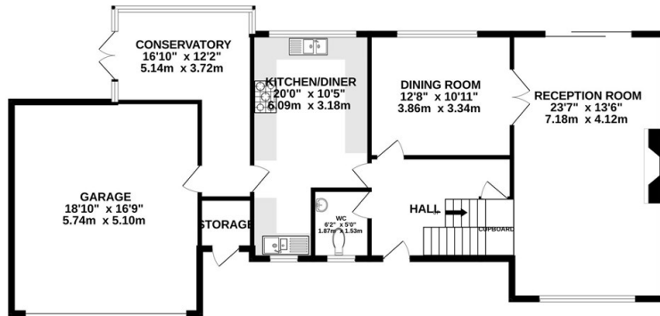
GROUND FLOOR 1247 sq.ft. (115.8 sq.m.) approx.
